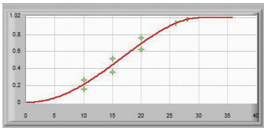
(Left) Plot of typical source showing compliance with the EF requirements in IEC 61280-4-1
